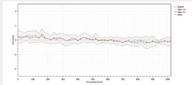
E.g. X Axis Laser Compensation under 5 microns.
