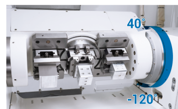
Tilting axis motion ranges
