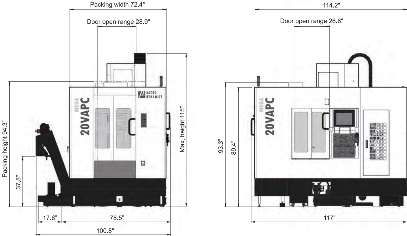
MACHINE DIMENSIONS Unit: inch
