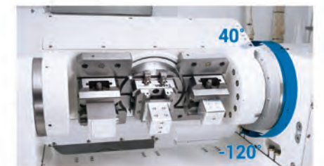
Tilting axis motion ranges
